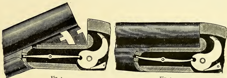
Greener's Emperor Hammerless Gun.
